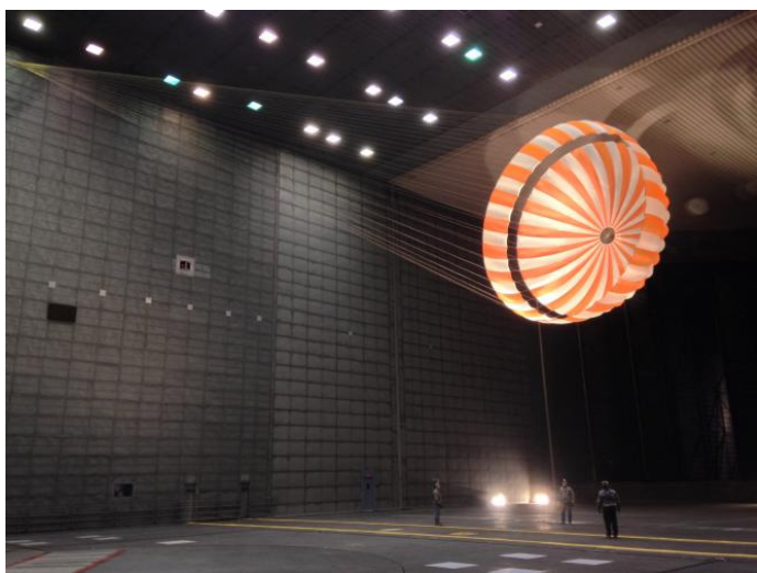
Parachute testing for InSight, conducted inside world's largest wind tunnel, at NASA Ames Research Center, Moffett Field, California.
